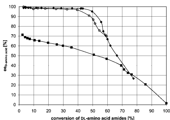
Figure 6. Enantioselectivity of the D-amidase as a function of conversion c of DL-Val-amide (♦), DL-Leu-amide (○) and DL-Phe-amide (■).
