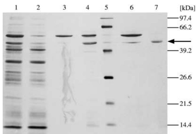
Figure 3. Purification of D-amidase from Variovorax paradoxus after HIC, analyzed by SDS-PAGE: IEC-pool (lane 1; 5 µg protein), flow through HIC (lane 2; 5 µg protein), fraction No. 6: 0.07 U/mg (lane 3, 2.5 µg protein), fraction No. 9: 0.2 U/mg (lane 4, 2.5 µg protein), marker proteins (lane 5), fraction No. 13: 0.8 U/mg (lane 6, 2.5 µg protein), fraction No. 17: 1.4 U/mg (lane 7, 2.5 µg protein). D-Amidase is indicated with an arrow. The gel was silver stained.
