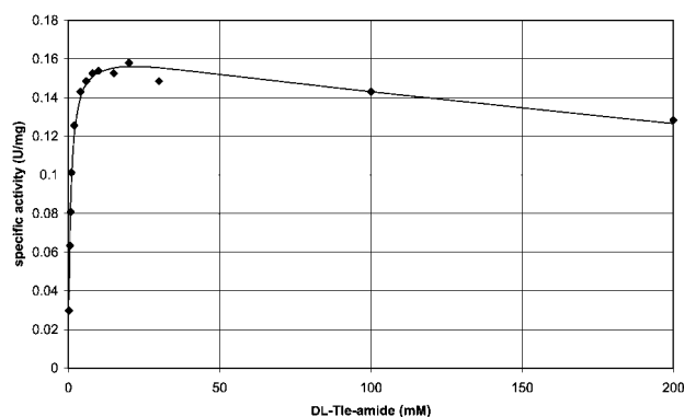
Figure 4. Michaelis–Menten plot for the conversion of DL-Tle-amide by the D-amidase from Variovorax paradoxus . Enzyme preparations after one chromatographic step were used with a specific activity of 0.16 U/mg.
