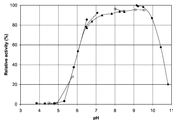
Figure 5. Optimum pH for the D-amidase activity. Levels of activity were determined by using the standard assay and the following buffers (each at a final concentration of 0.1 M): sodium citrate (●), sodium acetate (□), 2-( N -morpholino)ethanesulfonic acid (MES) (◆), potassium phosphate (▲), Tris-(hydroxymethyl)aminomethane (○), and sodium carbonate (♦). The activity for sodium carbonate buffer, pH 9.2, with 0.61 U/mg was taken as 100%.
